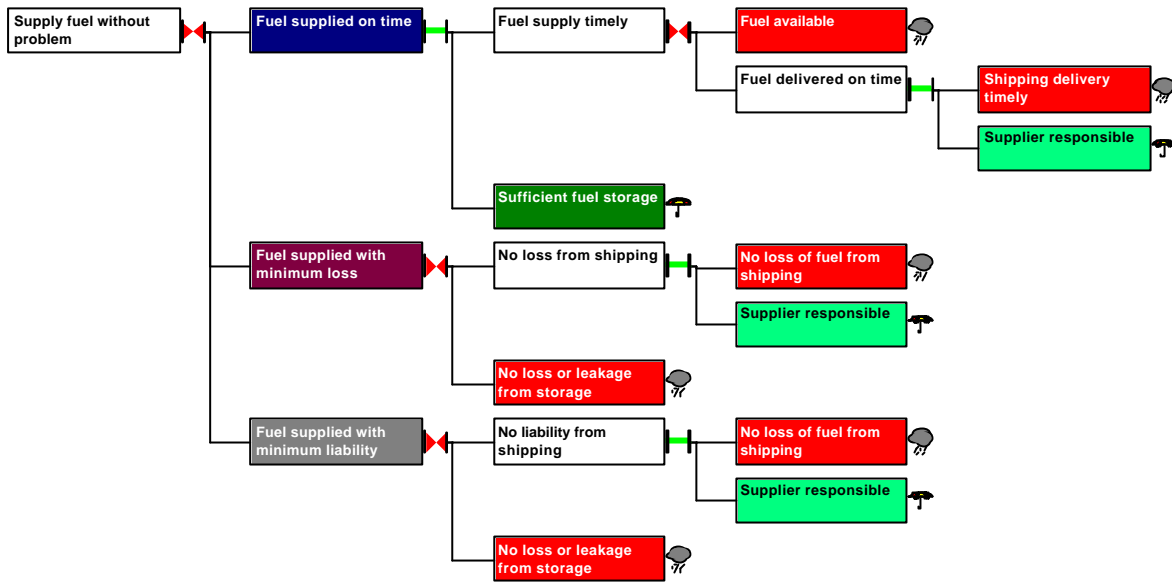
Figure 3 Dependency Map
