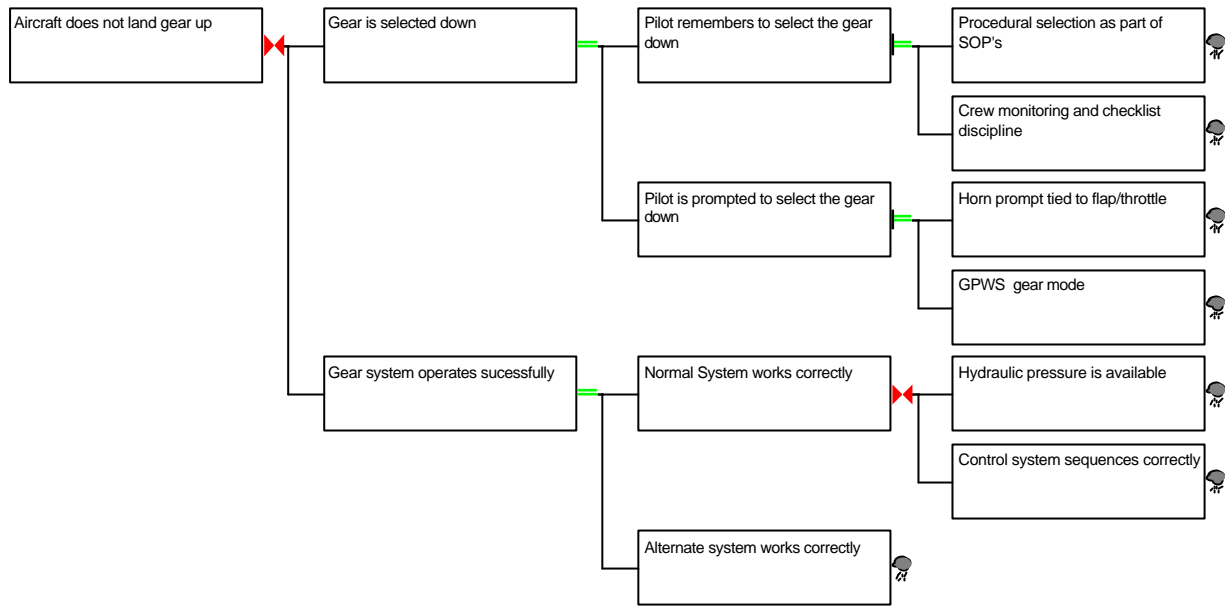
Figure 4 Dependency Model – Landing Gear
